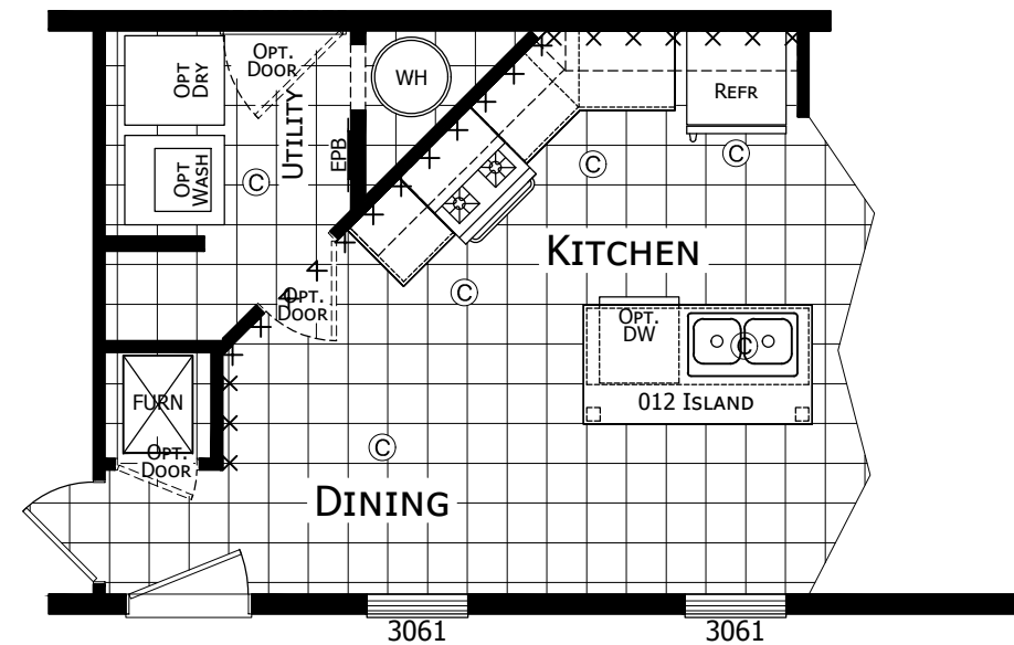
KITCHEN OPTION(REVERSE AISLE)
