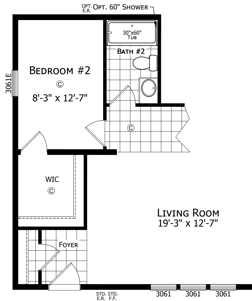
2 BEDROOM OPTION
