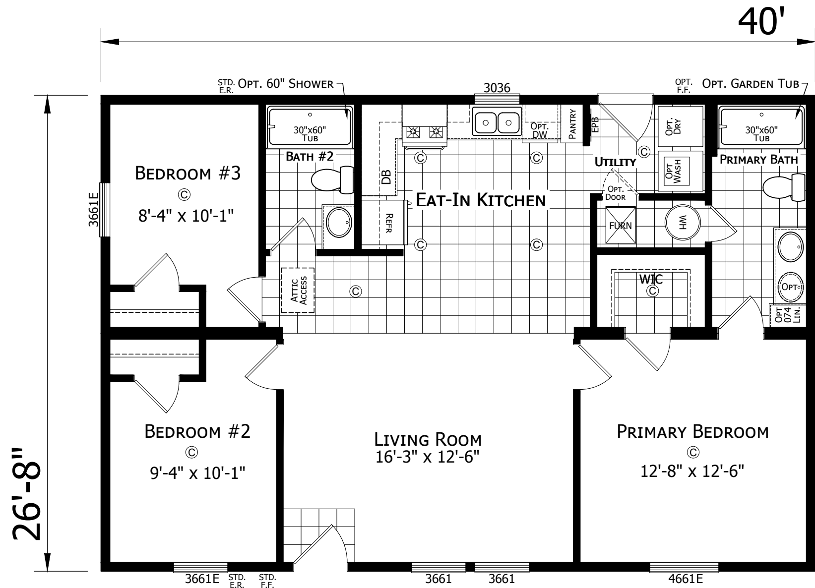
112APF-2840M32024 3 BEDROOM 2 BATH 40'-0" x 26'-8" 1067 Sq. Ft. TOTAL
