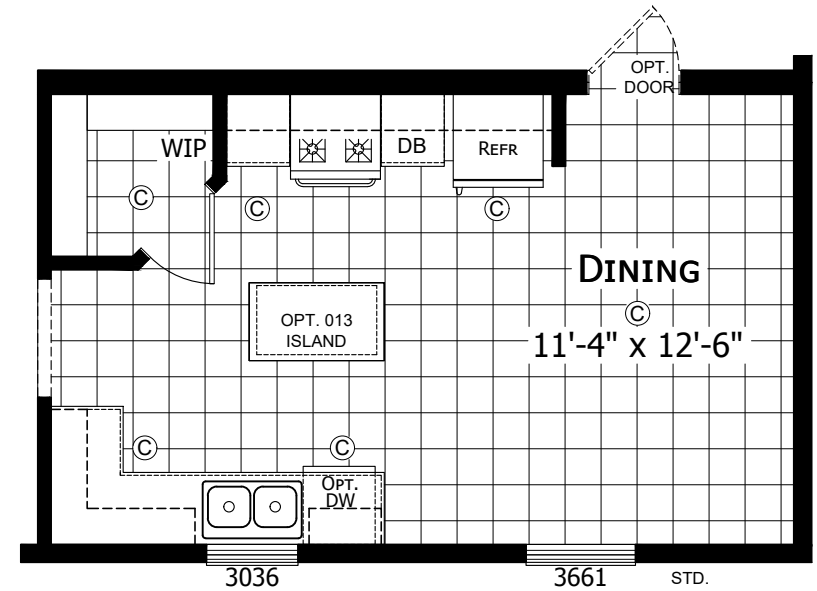
OPTIONAL KITCHEN #2
