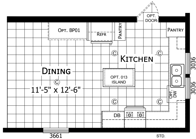
OPTIONAL KITCHEN #1
