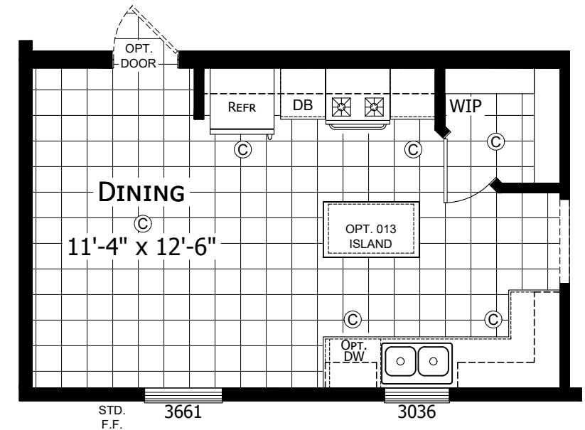
OPTIONAL KITCHEN #2
