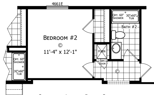
OPTIONAL LIVING ROOM OFFSET
