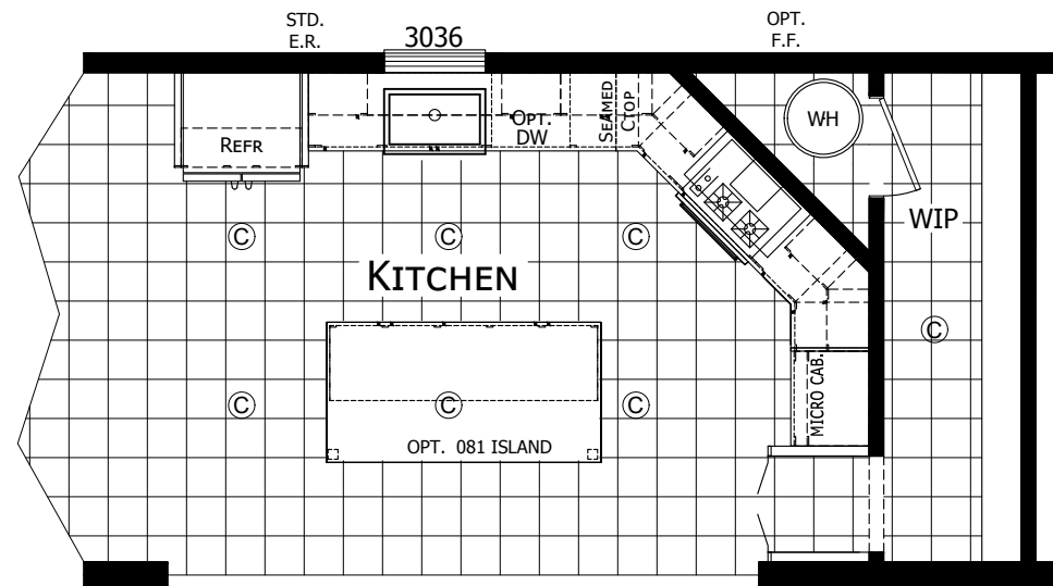
OPTIONAL ULTIMATE KITCHEN II
