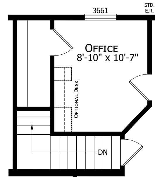
OPTIONAL STAIRWELL N/A W/ OPTIONAL 4TH BEDROOM
