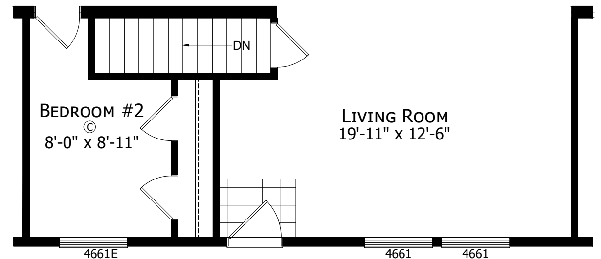
STAIRWELL OPTION
