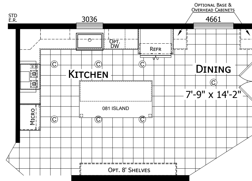
OPTIONAL ULTIMATE KITCHEN #2
