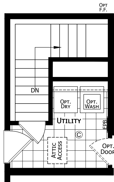
OPTIONAL STAIRWELL NO FURNACE AND W/H INCLUDED
